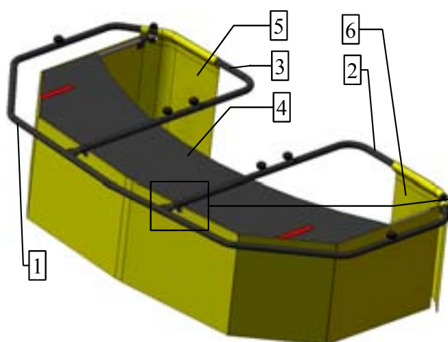
Obr. 2: Ochranná plachta
